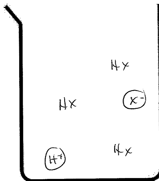
Dilute Weak Acid
