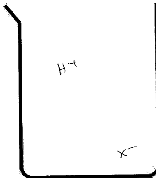
Dilute Strong Acid
